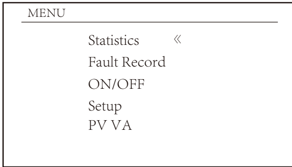
Figura 8.6 Menu Principal
