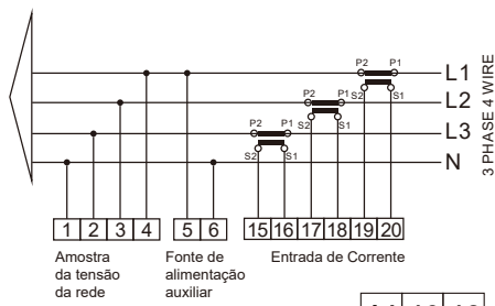
Eastron SDM630MCT Figura 7.12 Medidor Eastron
