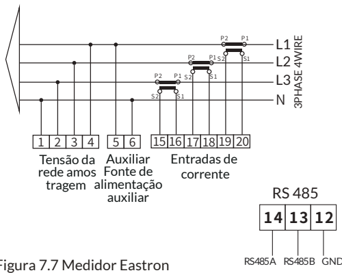
Eastron SDM630MCT
