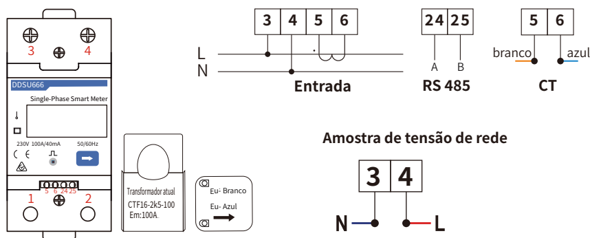
DDSU666-CT (CTF15-2K5-100A)
