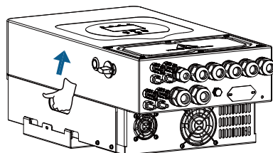
SUN-(7-10)K-SG05LP1-EU-AM2-P
