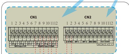
Inversor
